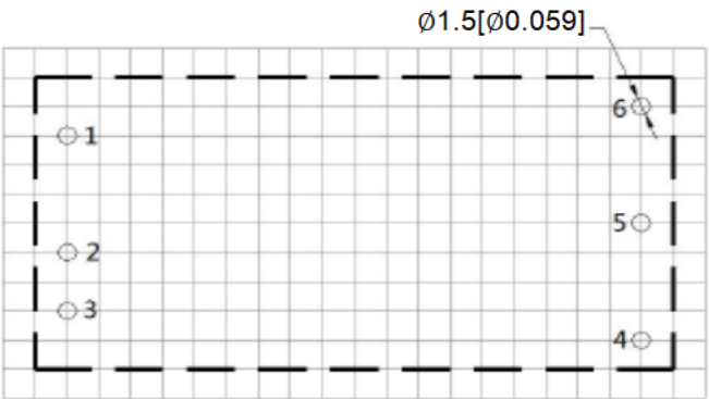
栅格距离2.54*2.54mm
